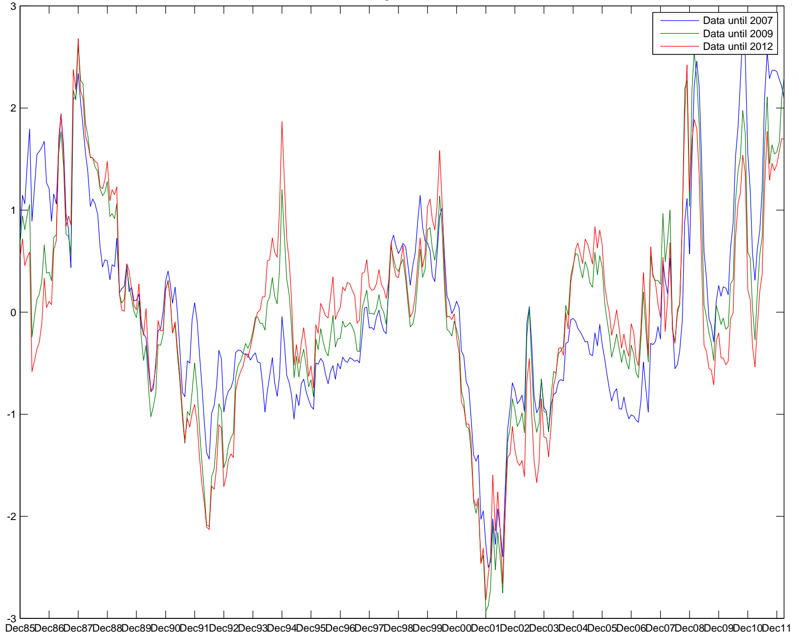
Standardizing the filtered series
